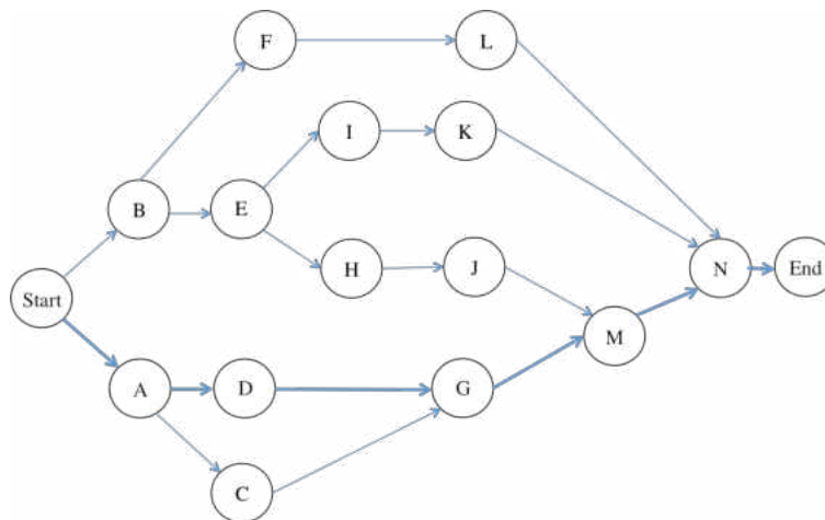
Figure 4.1: Case Study Network
