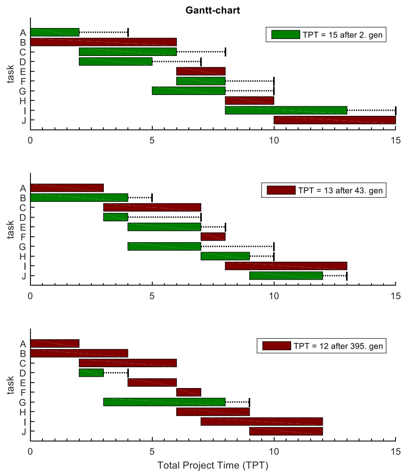
Figure 5.3: Gantt Charts
