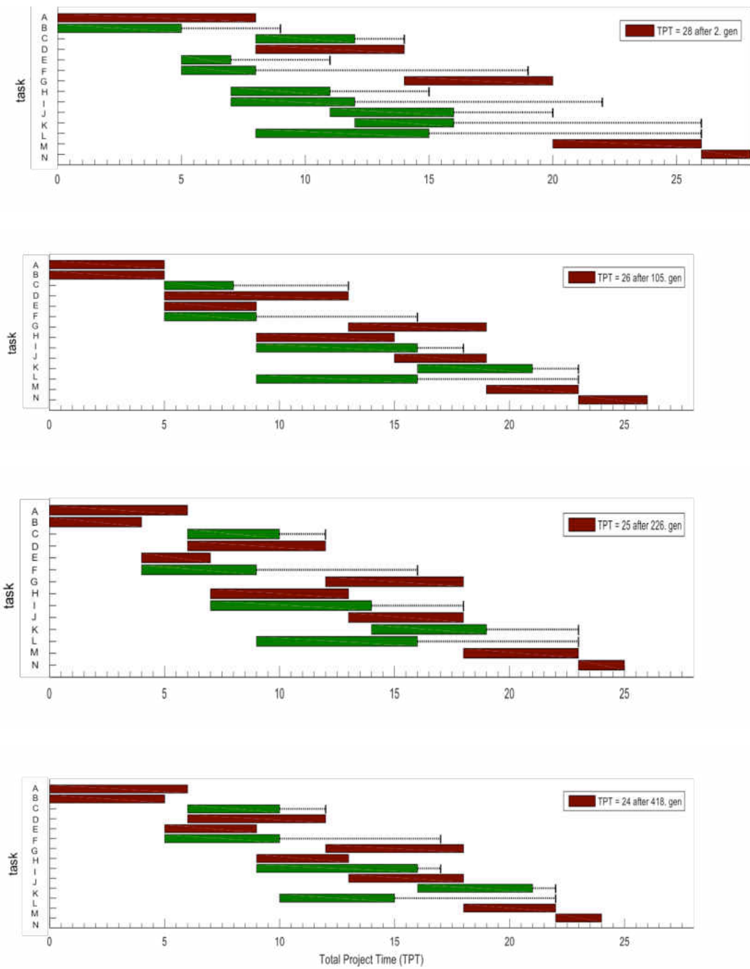
Figure 4.5: Gantt Charts
